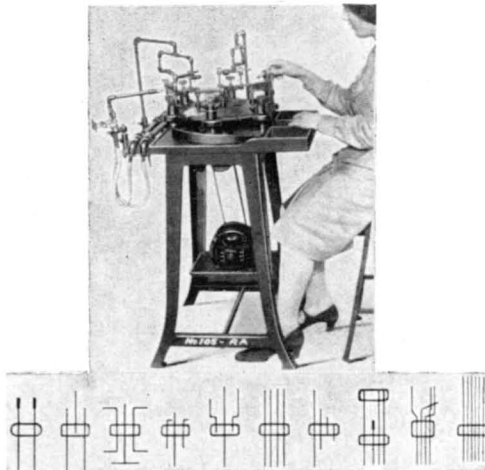
The Eisler glass-bead machine (Patent No. 1,866,634) and the various types and shapes of beads produced.
